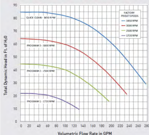
PERFORMANCE CURVES - MAX-E-PROXF VS COMMERCIAL PUMP
