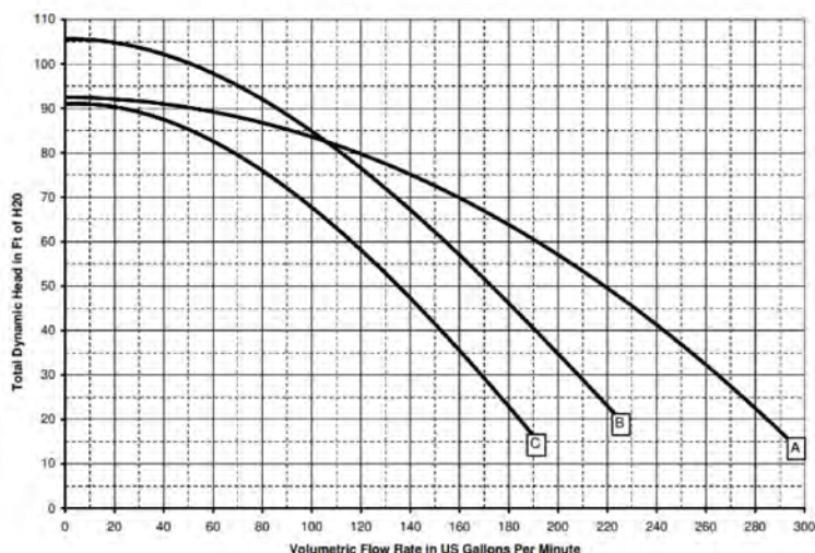
Pump Performance Curves
